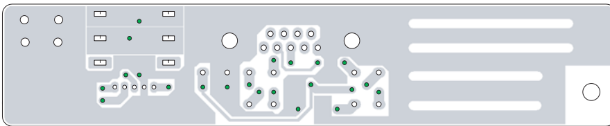
U2:NAETC-7347 (Bottom Side View from Top Side)
